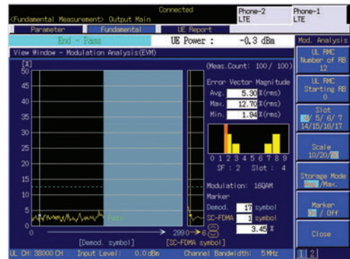
Transmitter Measurement (EVM)
