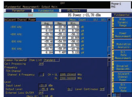
Adjacent Channel Power
