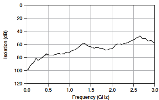
Figure 4. Isolation, Typical
