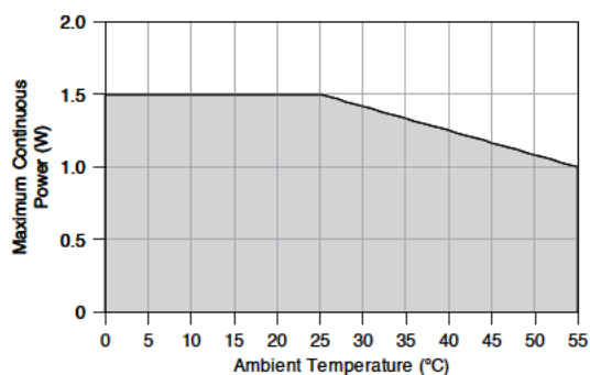
Figure 5. Termination Derating
