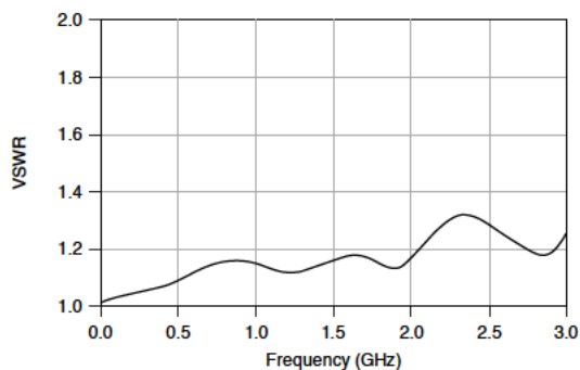
Figure 3. Termination VSWR, Typical
