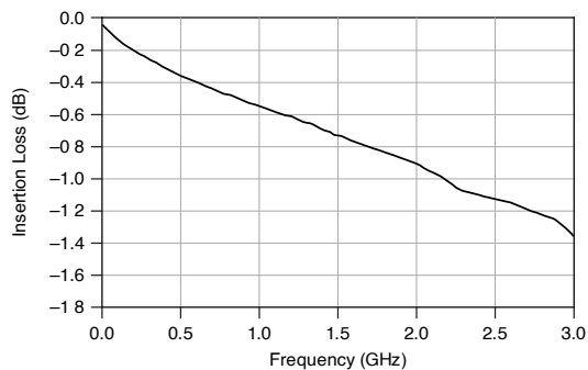
Figure 1. Insertion Loss, Typical
