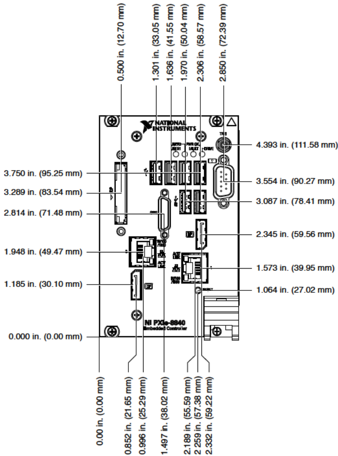
Figure 1. PXIe-8840 Front Panel Layout and Dimensions
