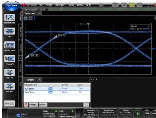
Figure 2. Output eye showing rise time < 12 ps.
