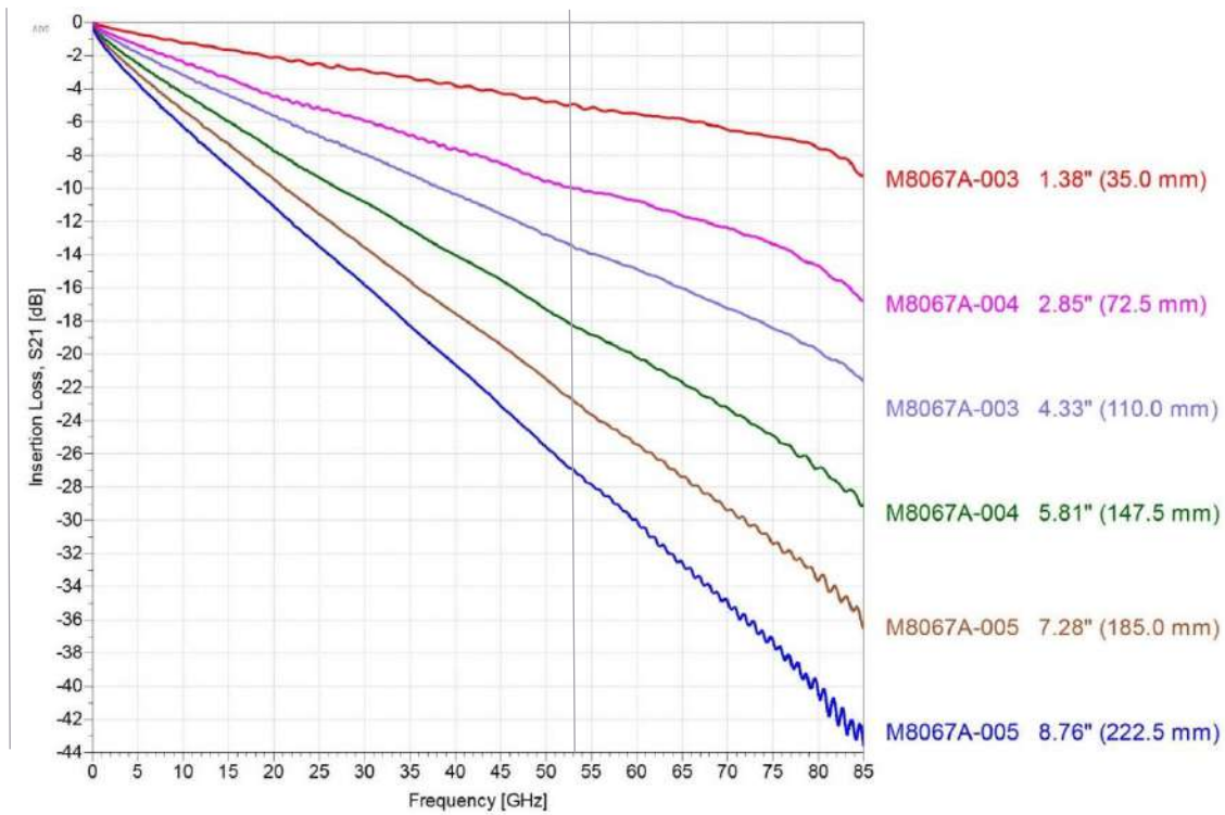
Figure 7. Typical insertion loss of ISI channel board M8067A-003, -004, and -005 with 1.0 mm connectors.
