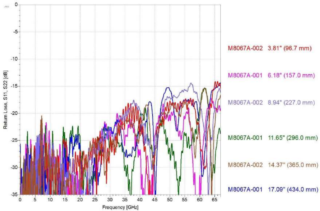
Figure 6. Typical return loss of ISI channel board M8067A-001 and -002 with 1.85 mm connectors.
