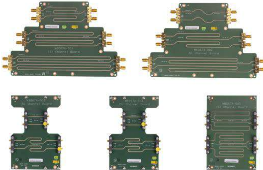
Figure 2. Front view of ISI channel boards without brackets. The M8067A option -001, -002 ISI channel boards shown in the top row have 1.85 mm connectors and the M8067A-003, -004, -005 ISI channel boards shown at the bottom have 1.0 mm connectors.
