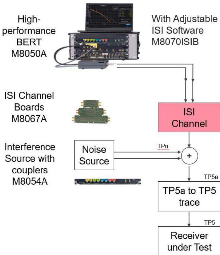
Figure 1. Typical receiver test setup with M8050A high-performance BERT, interference source and ISI channels.
