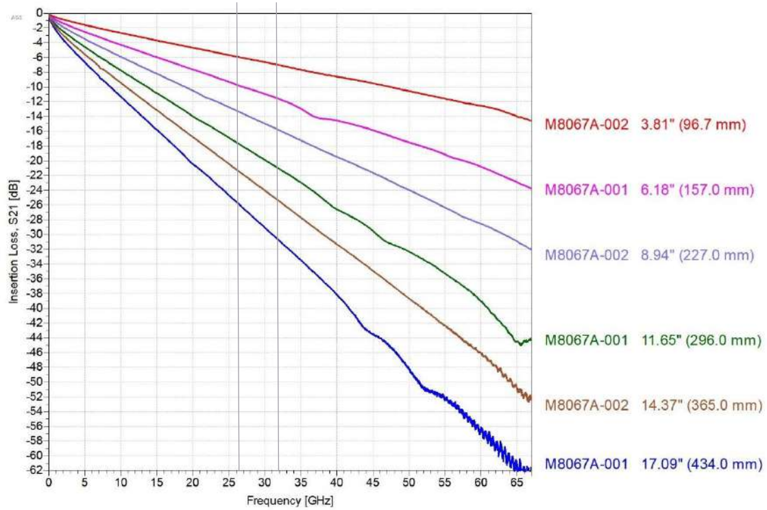
Figure 5. Typical insertion loss of ISI channel board M8067A-001 and -002 with 1.85 mm connectors.
