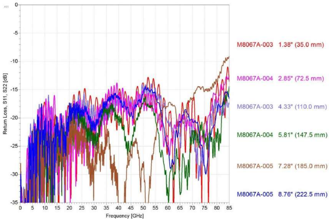
Figure 8. Typical return loss of ISI channel board M8067A-003, -004, and -005 with 1.0 mm connectors.
