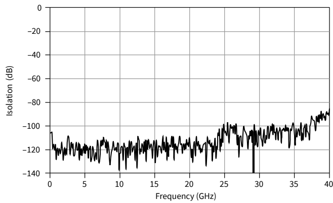
Figure 2. Typical Isolation
