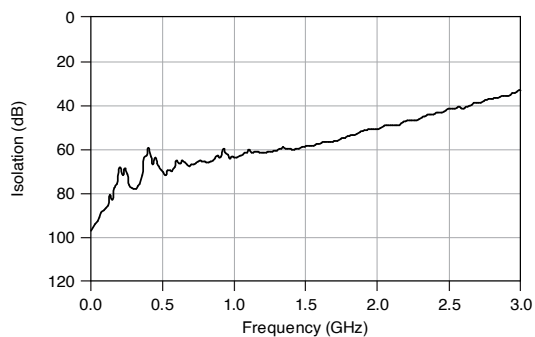
Figure 3. Isolation, Typical
