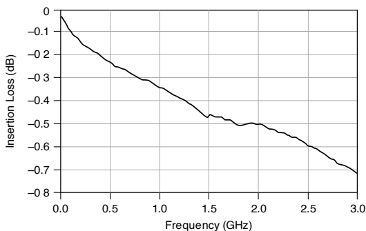
Figure 1. Insertion Loss, Typical
